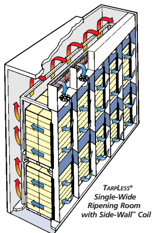
Two-tier, 44 pallet TarPless® ripening Rooms with Side-Wall™ cooling coils. Safeway - Portland, Oregon.
